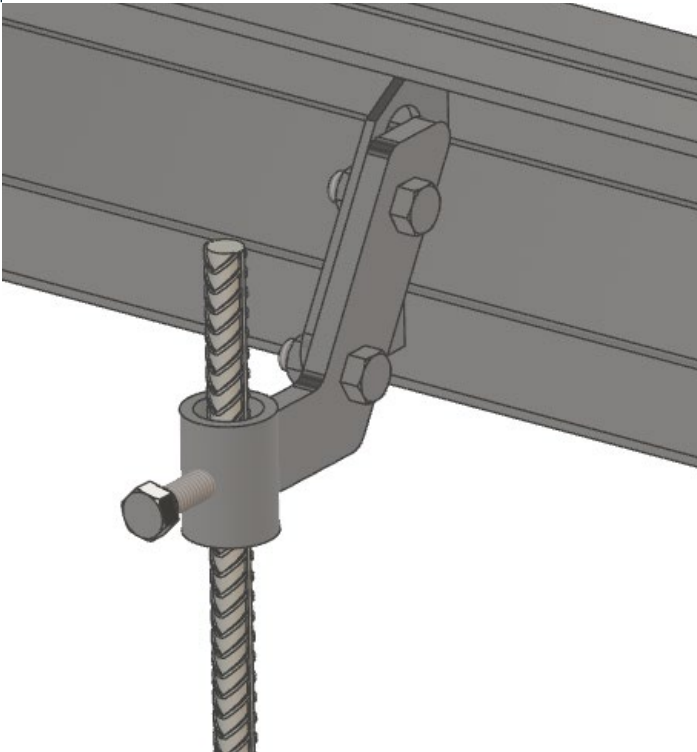
Adjustable height Bracket, Number of staking brackets, customizable Hose barb for trough flushing water line
