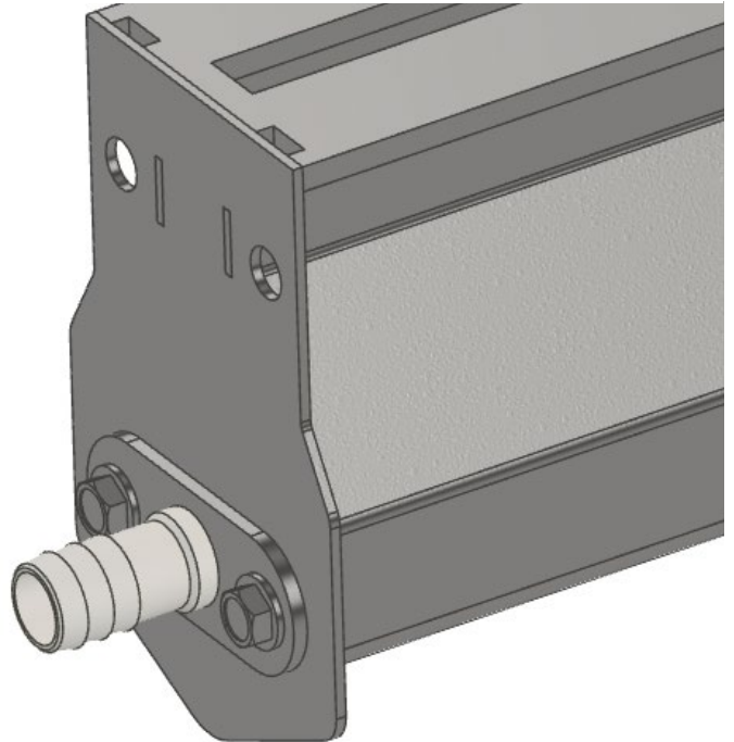
Adjustable height Bracket, Number of staking brackets, customizable Hose barb for trough flushing water line
